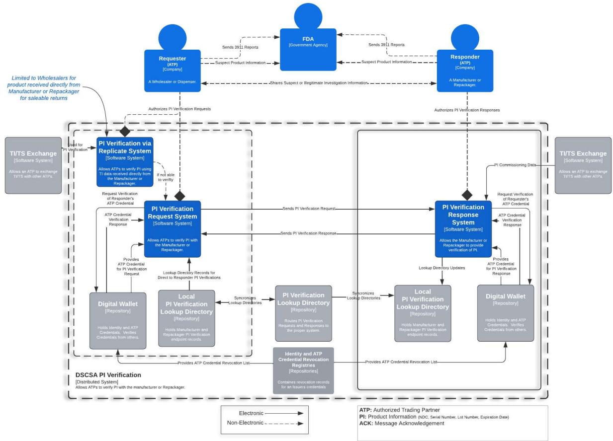
Figure 2 – PI Verification without the need to route the request to another VRS solution.
