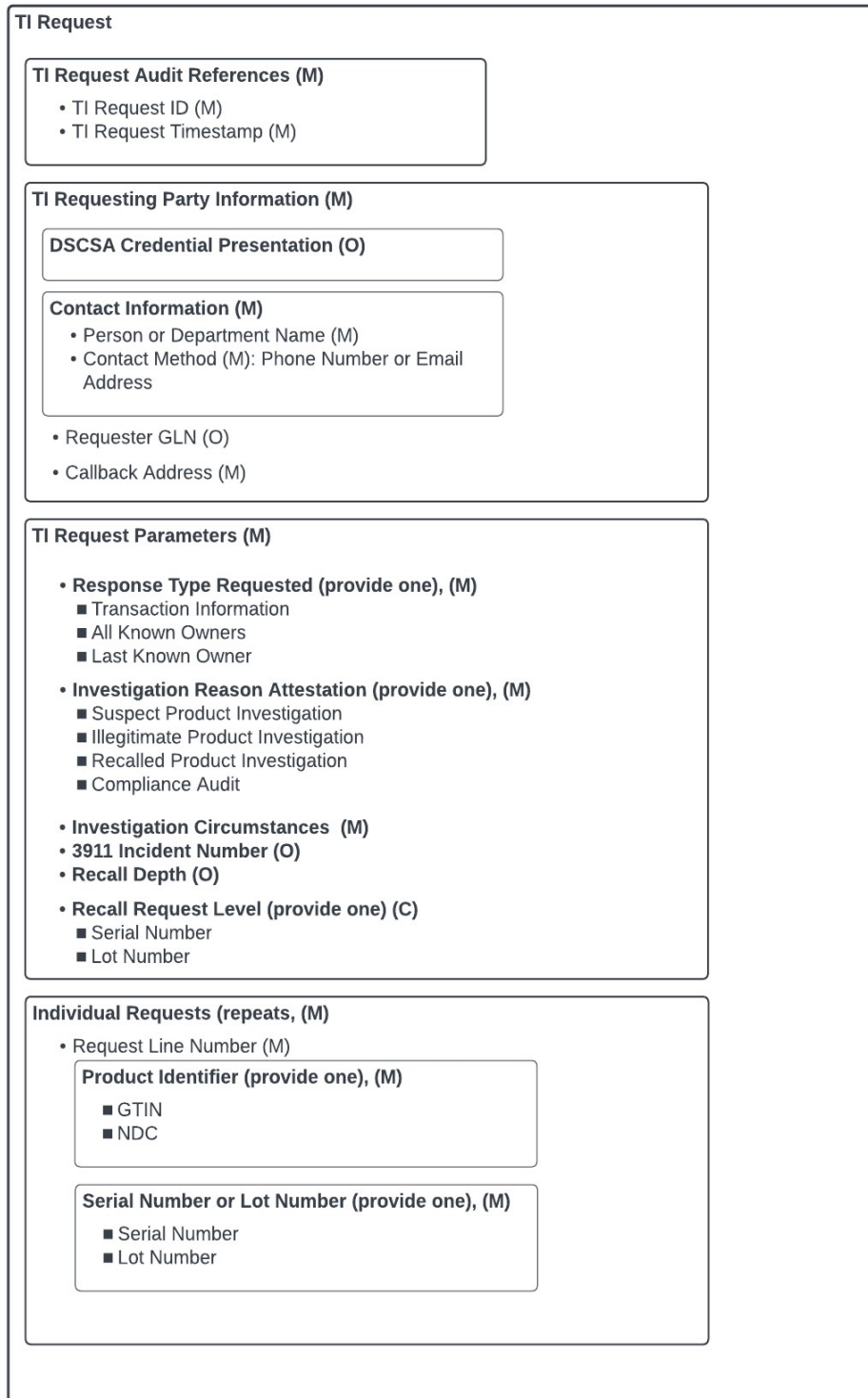
Figure 7 – Detail of TI Request Message Structure
