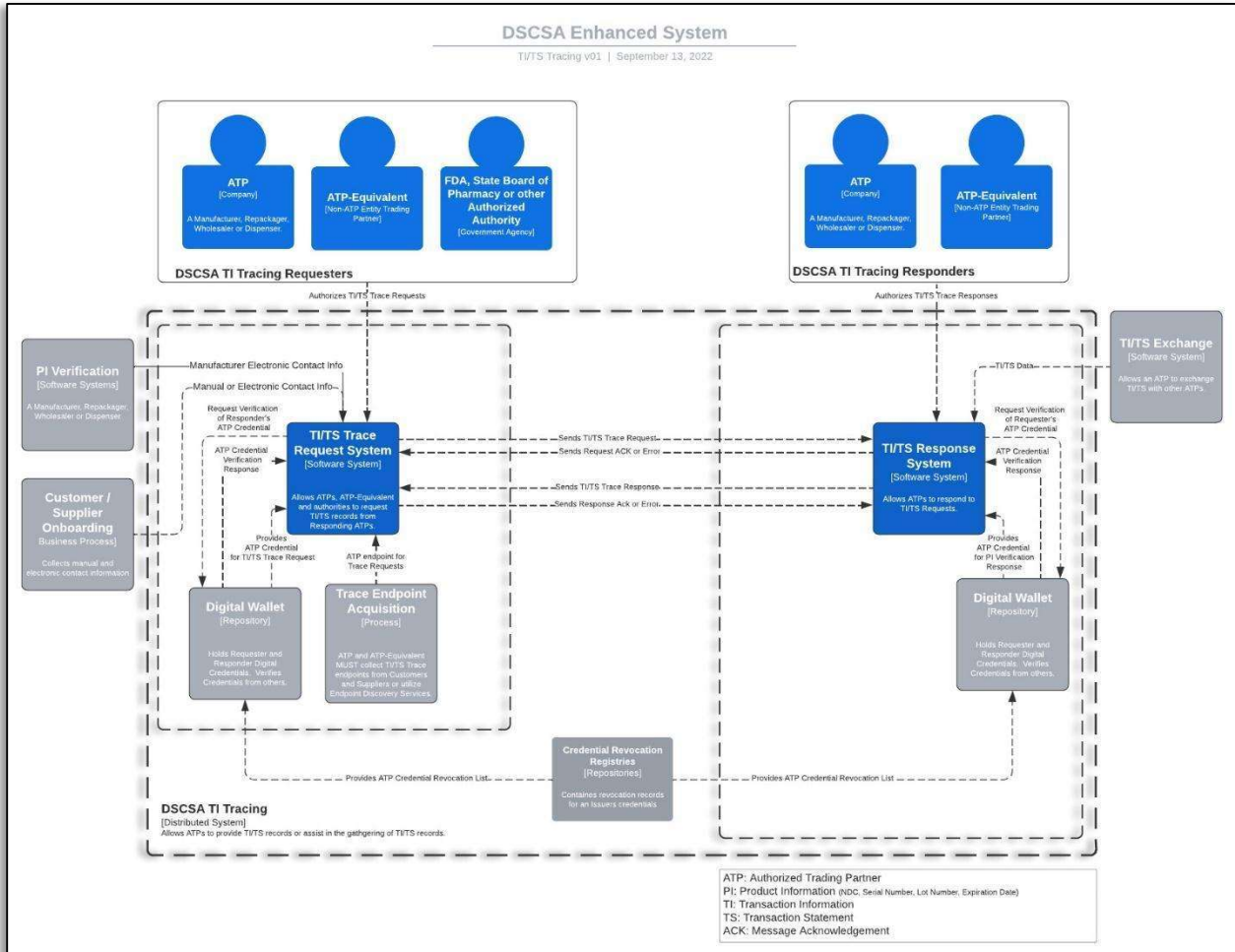
Figure 2 - TI/TS Trace Request and TI Response
